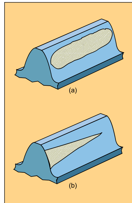
Figure 1 — Typical gear tooth contact patterns: (a), aligned, and (b), misaligned.
