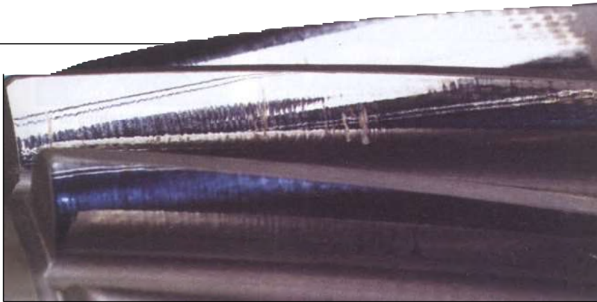
Figure 7 — Polishing type wear.
