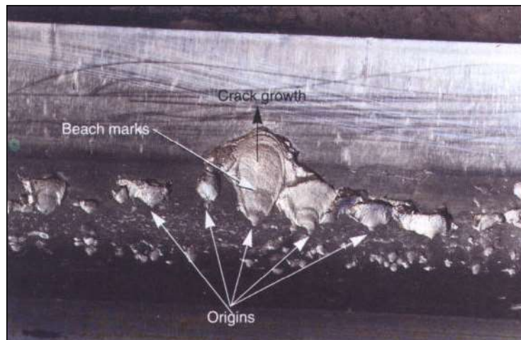
Figure 4 — Fatigue failure (pitting) in the contact surface of a gear tooth. Beach marks are visible in some of the larger pits.
